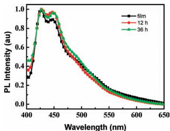
Figure 4. PL spectra of BLHPC in film before and after annealing at 150 °C in air.
