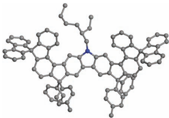
Figure 1. Optimized molecular structure of BLHPC calculated with PM3.
