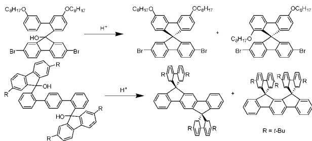
Scheme 1. Positional Isomers Generated in Ring-Closure Reaction
