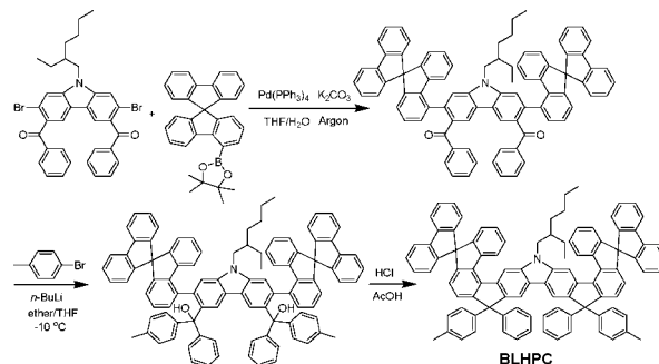
Scheme 2. Synthesis of BLHPC
