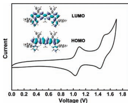
Figure 2. Cyclic voltammogram of BLHPC (inset: distribution of the HOMO and LUMO levels from DFT calculation of BLHPC).
