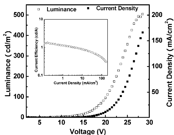
Figure 5. J – V – L curves of the device. (Inset: the current efficiency–current density curve of the device.)
